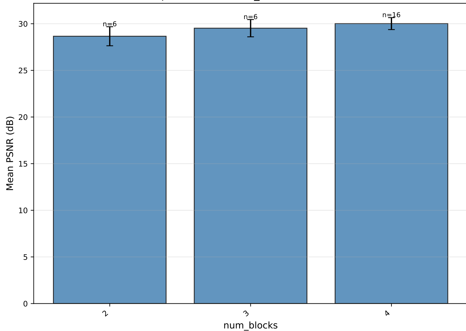
Mean PSNR per value of num_blocks — WaveletAttention
